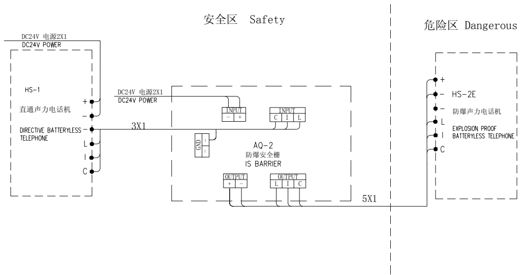
20: 防爆直通声力电话机接线图 Explosion-proof interphone batteryless telephone set connection diagram
